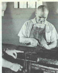
Six milled segments are immersed in Bakelite cement, and then cross wrapped under tension to form a hexagonal section in which the seams are invisible.
